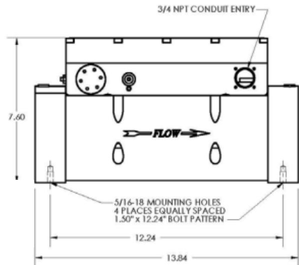
Model AGV Installation View
