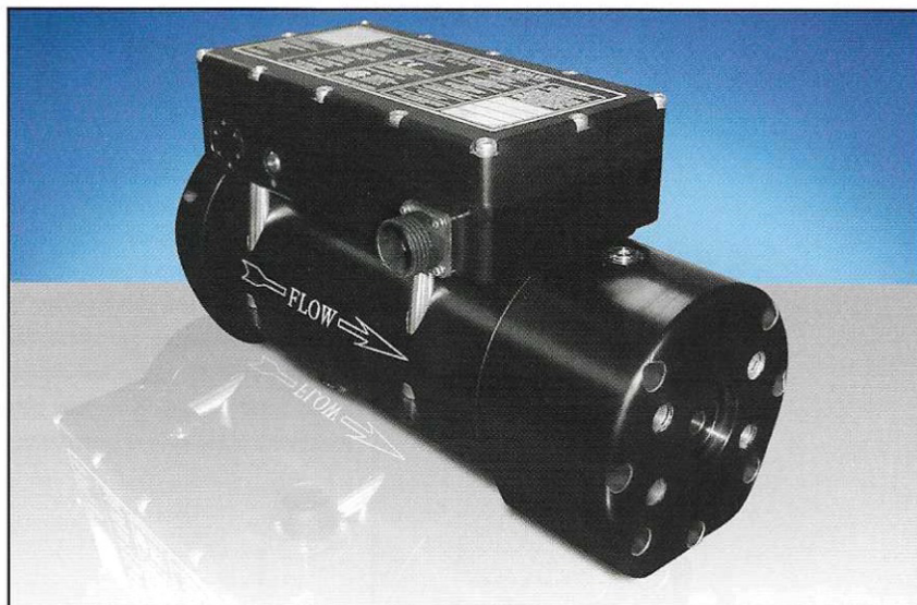
The AGV50 Pilot gas valve for gas turbines in low NO x applications is designed for the precise flow requirements of such applications.
